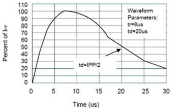
FIGURE 1 Pulse Waveform
